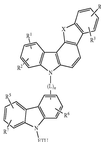
[Chemical Formula 2]
