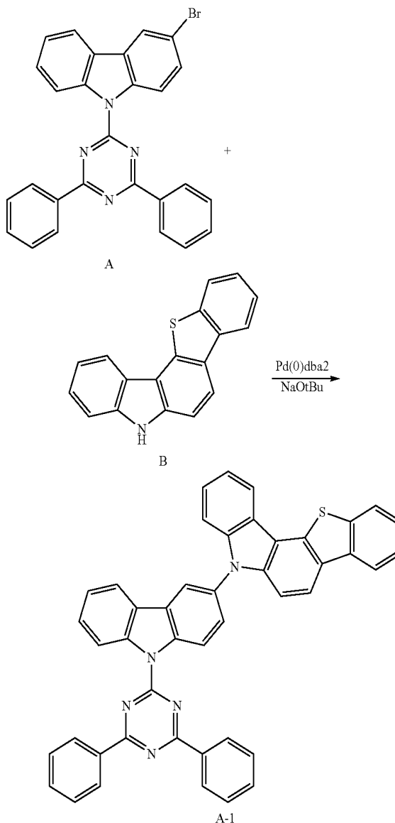
[Reaction Scheme 1]
